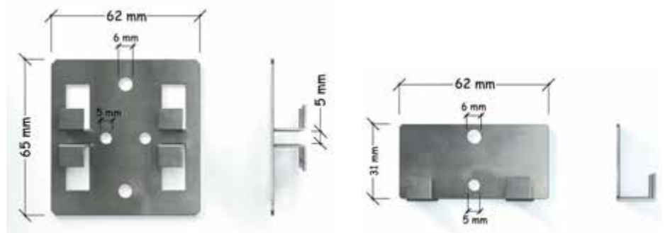
ART. CPKC G4 F4 Placca Intermedia Tipo 1 Intermediate plate Type 1
