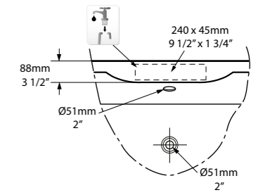
Rim Detail
