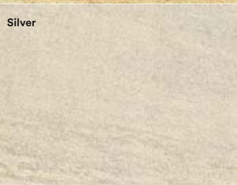
Gneiss
